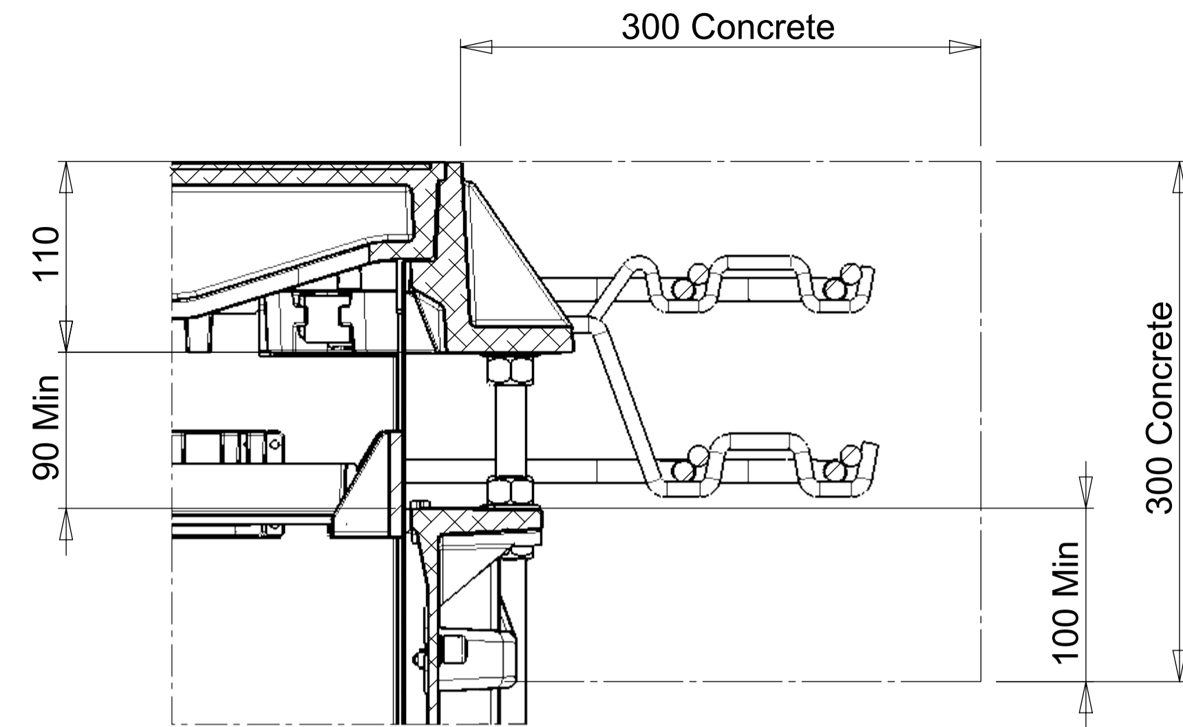
Concrete Collar
