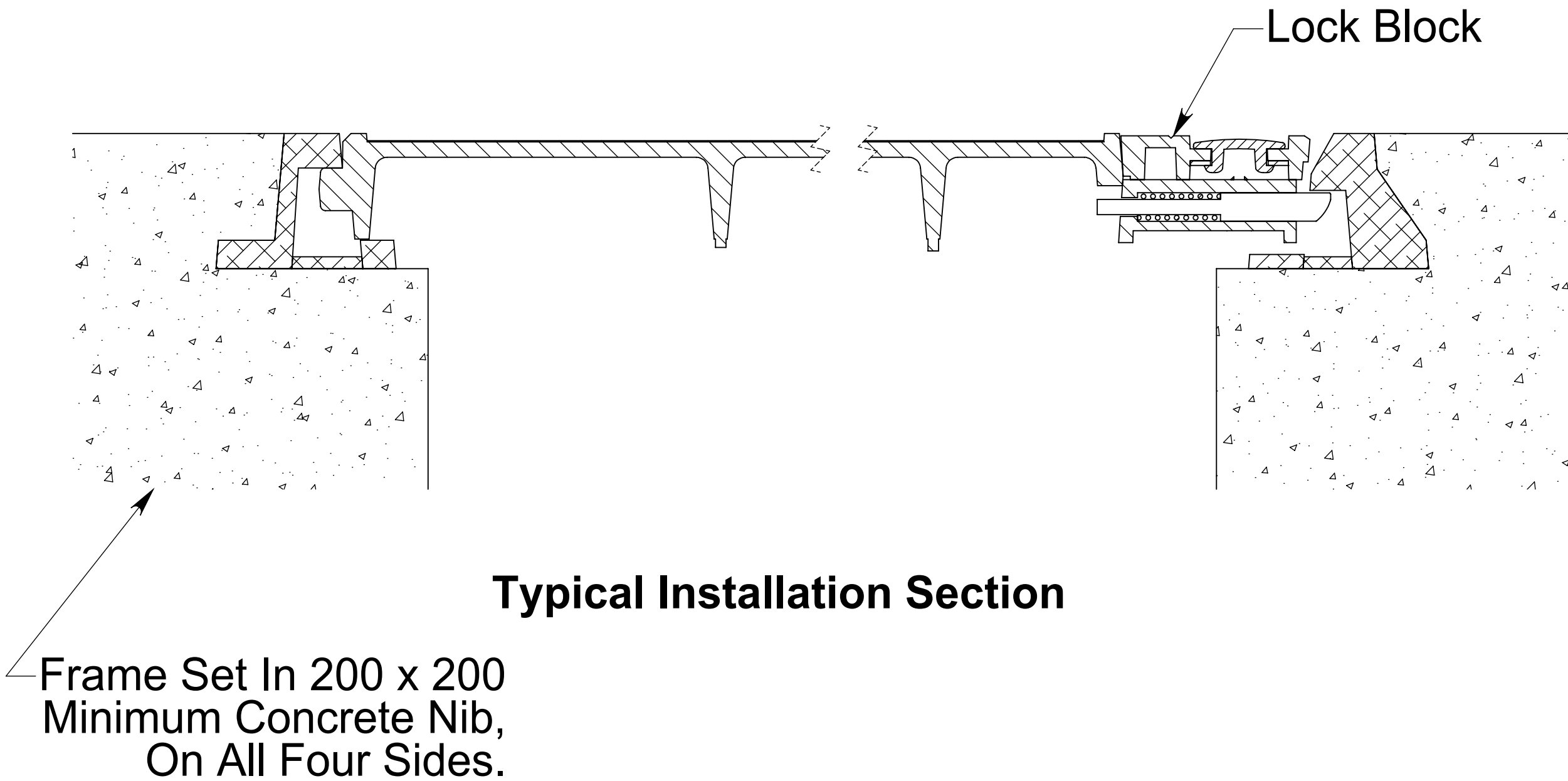
Typical Installation Section
