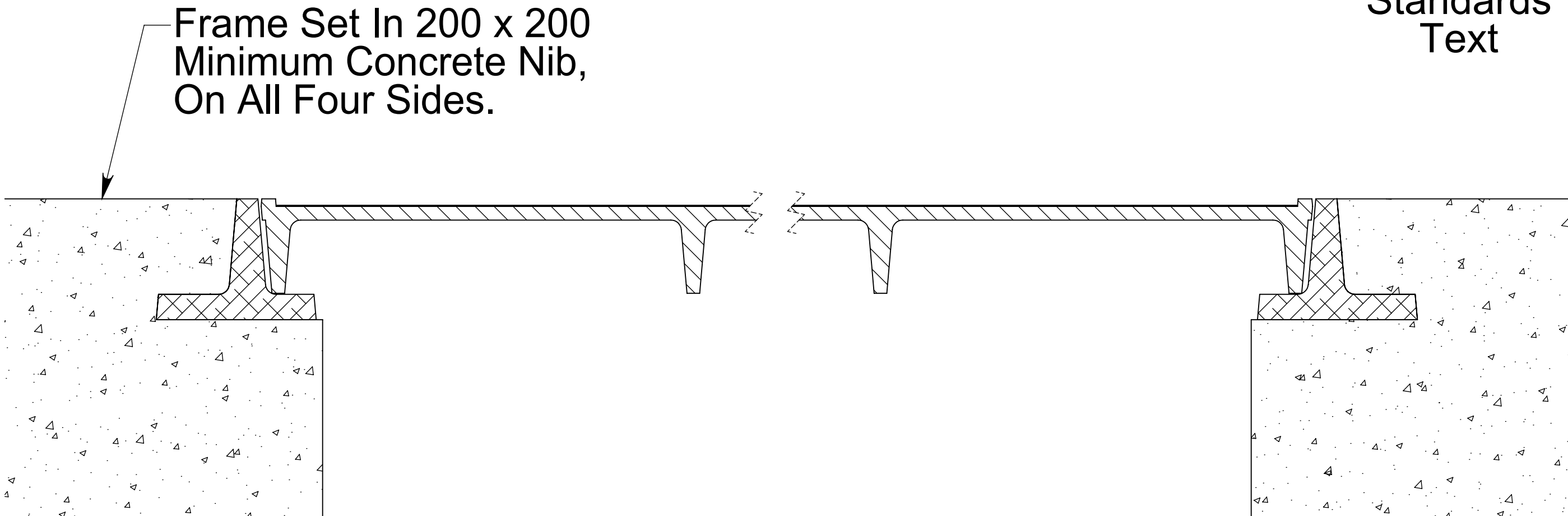
Typical Installation Section
