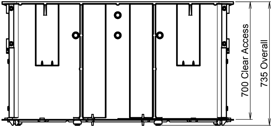
Side Elevation
