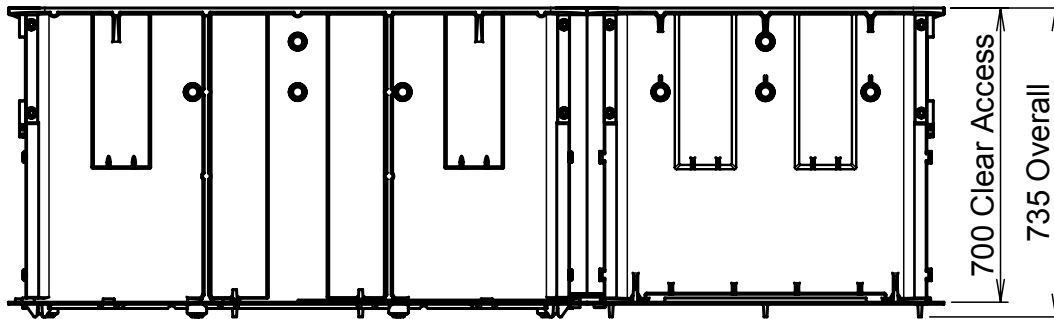
Side Elevation
