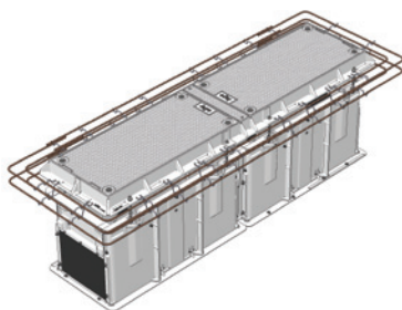
CLASS D CHAMBER AND COVER SET PACKAGE 2600 X 600 X 700H
