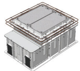
CLASS D CHAMBER AND COVER SET PACKAGE 2100 X 1200 X 700H
