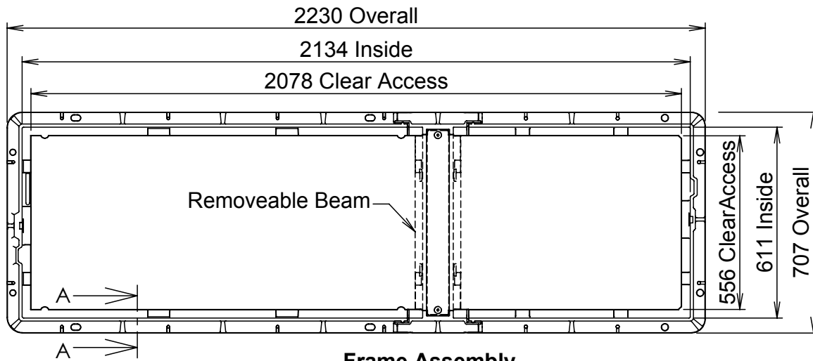
Frame Assembly
